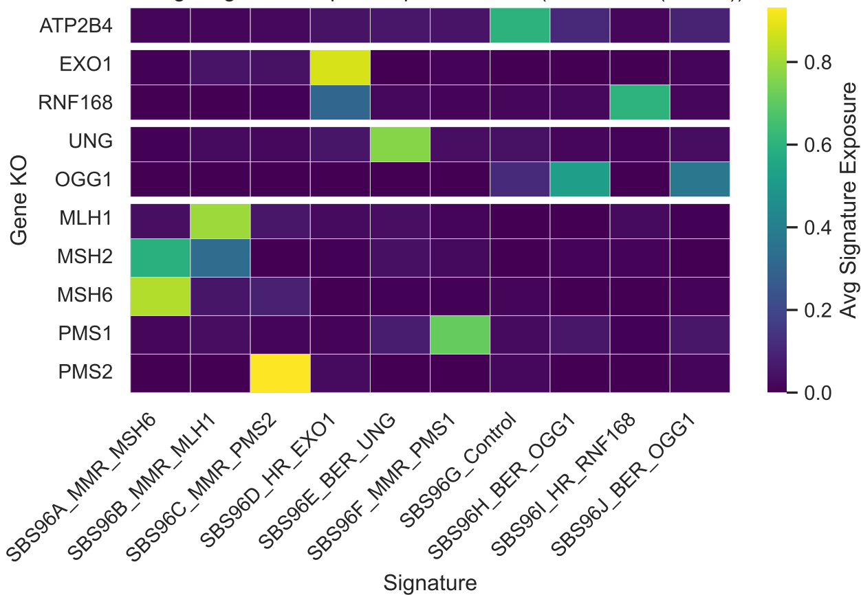
Average Signature Exposure per Gene KO (Gene level (K = 10))
